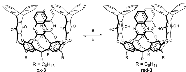
Figure 5. Redox interconversion between the quinone and hydroquinone states of cavitand 3 . a) \text{H}_2 , Pd/C, THF (degassed), 25 °C, 30 min, quantitative. b) Air, quantitative.
