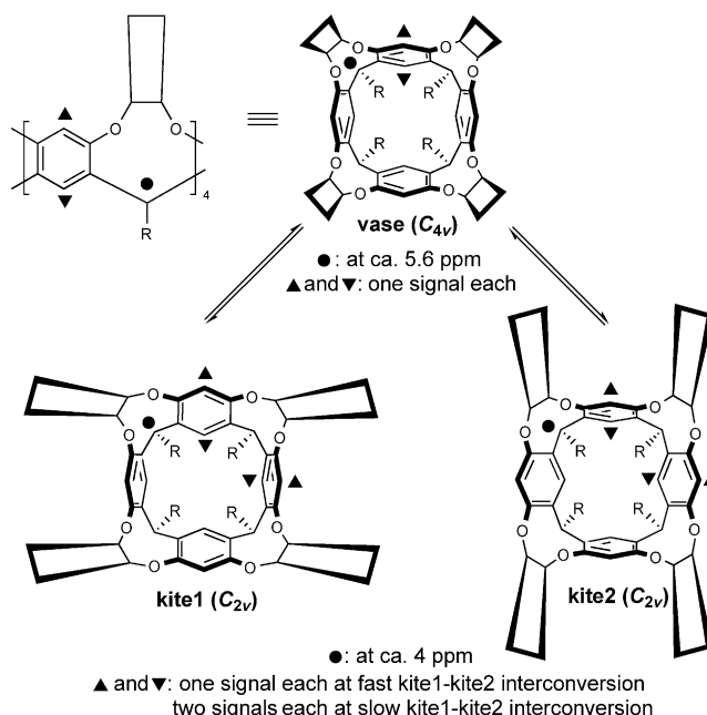
Figure 1. Vase–kite1–kite2 equilibrium of a generic cavitant and summary of characteristic 1 H NMR features of three situations: vase, kite with slow kite1–kite2 interconversion, and kite with fast kite1–kite2 interconversion.
