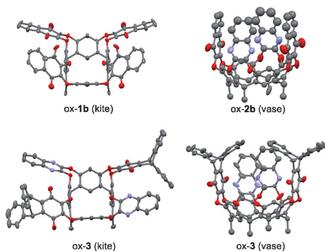
Figure 3. Crystal structures of cavitands ox-1b (top left, from acetone), ox-2b (top right, from DMF), ox-3 (bottom left, from [\text{D}_{12}]\text{mesitylene} ), and ox-3 (bottom right, from DMF) at 100 K. Solvent molecules, n -hexyl chains, and hydrogen atoms are omitted for clarity. Thermal ellipsoids are shown at the 50% probability level.
