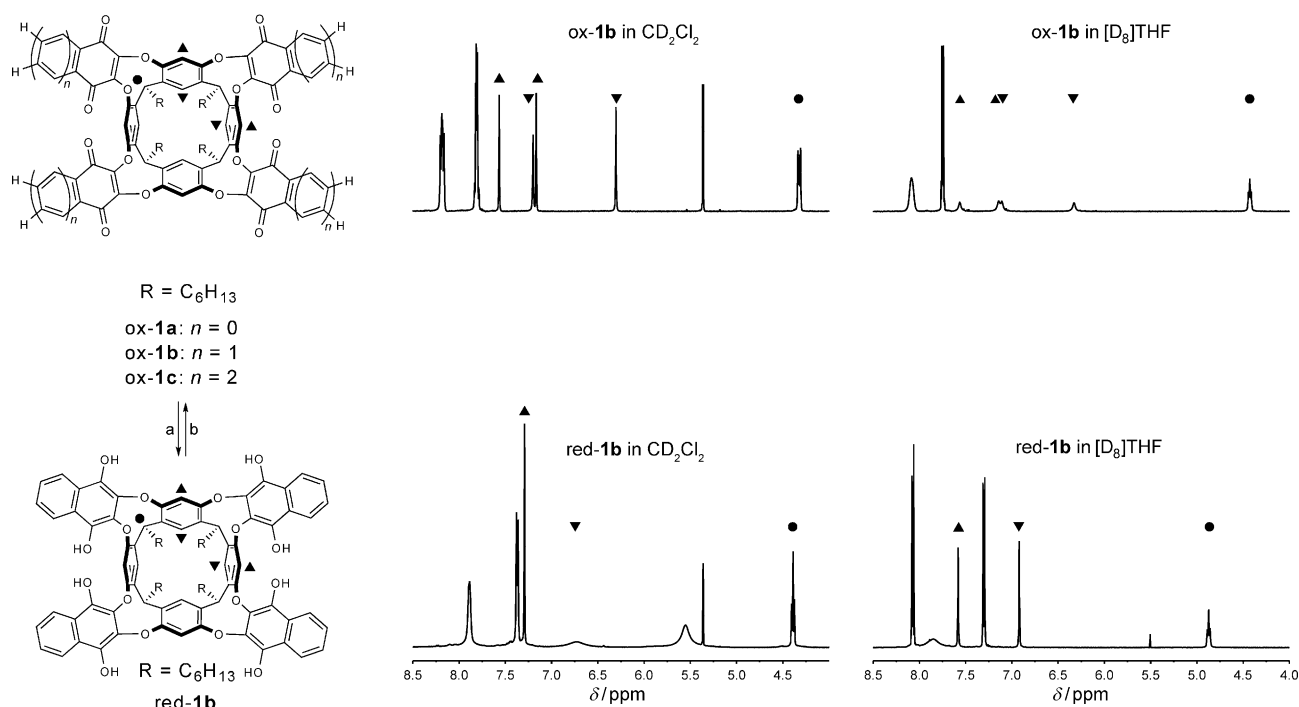
Figure 2. Left: Cavitands ox-1a-c and redox interconversion between the quinone and hydroquinone states of cavitand 1b . a) \text{Na}_2\text{S}_2\text{O}_4 , \text{CDCl}_3/\text{H}_2\text{O} (degassed), 60^\circ\text{C} , 3 h, quantitative. b) Air, quantitative. Sections of the ^1\text{H} NMR spectra (298 K, 500 MHz) of cavitands ox-1b and red-1b in \text{CD}_2\text{Cl}_2 (middle) and [\text{D}_8]\text{THF} (right).
