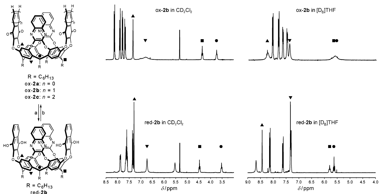
Figure 4. Left: Cavtands ox-2a–c and redox interconversion between the quinone and hydroquinone states of cavtand 2b. a) Na 2 S 2 O 4 , CDCl 3 /H 2 O (degassed), 60 °C, 3 h, quantitative. b) Air, quantitative. Sections of the 1 H NMR spectra (298 K, 300 MHz) of cavtands ox-2b and red-2b in CD 2 Cl 2 (middle) and [D 8 ]THF (right).
